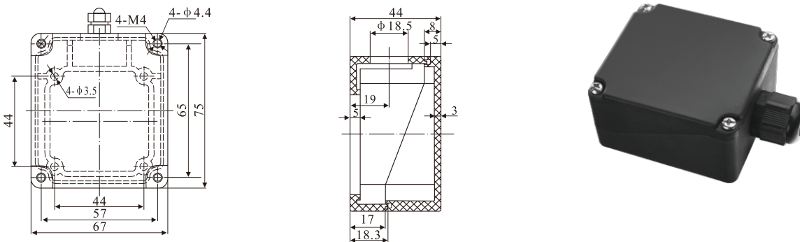
T2: SX型接線盒 T2: SX type junction box
