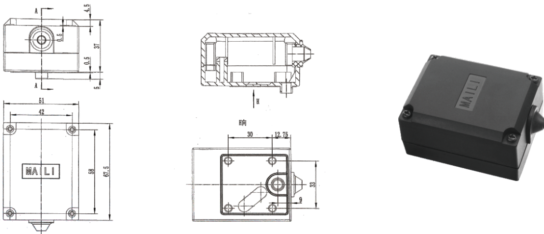
T1:ML接線盒 T1: ML junction box
