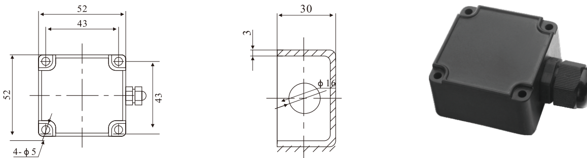
T3: 防水接線盒 T3: Waterproof junction box
